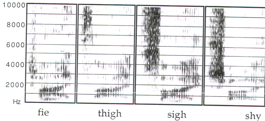
Figure 6.6. Acoustic structure of words with voiceless fricatives
