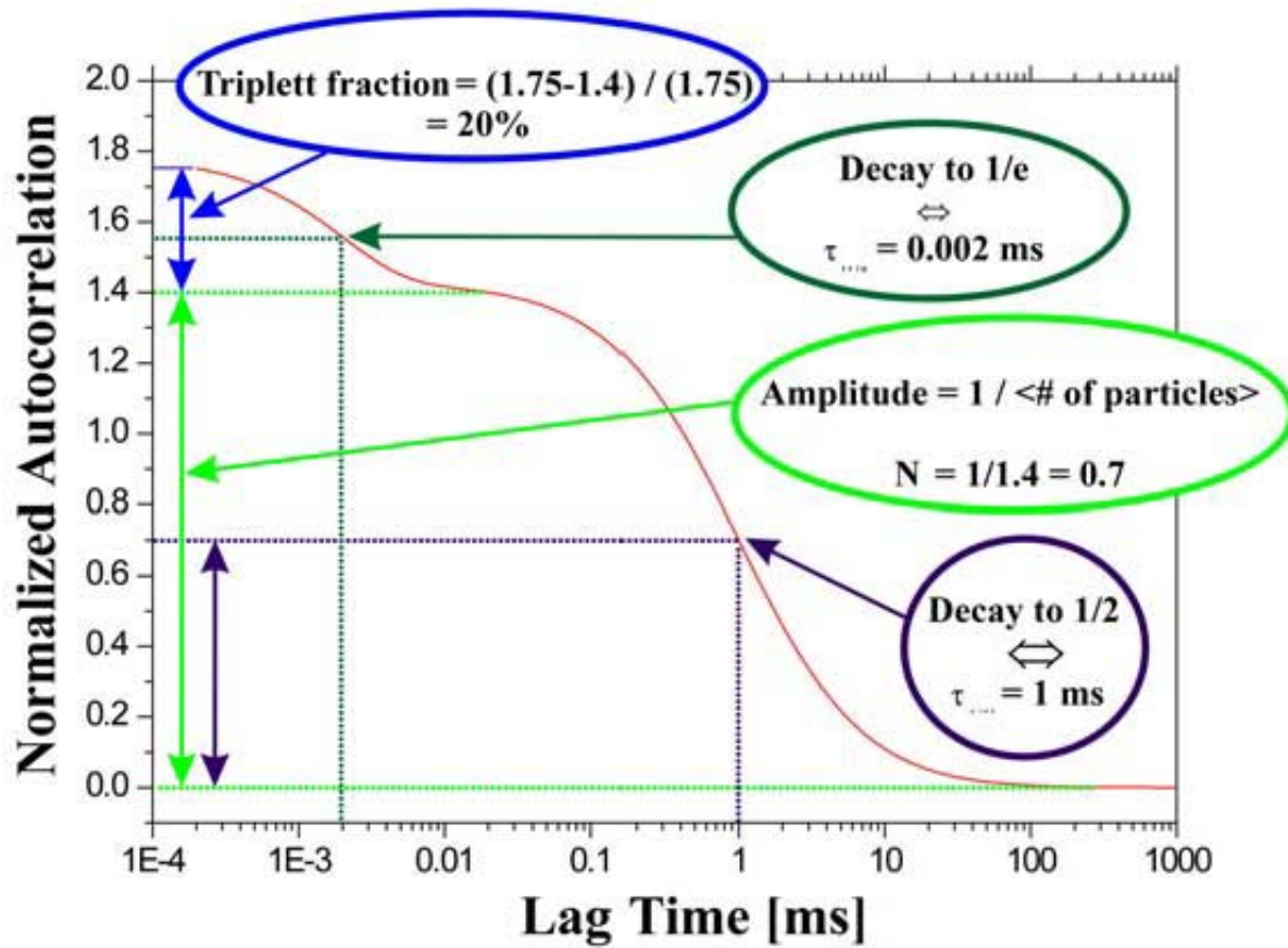
Autocorrelation curve with fast triplet dynamics
