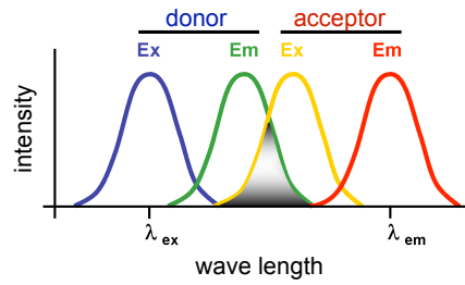
Figure 5: Schematic spectra of a donor-acceptor pair
