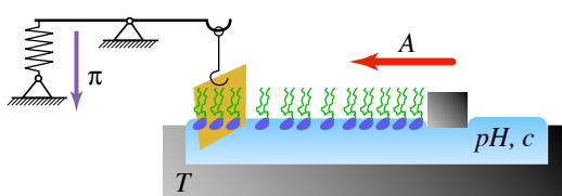
Figure 2: Sketch of a film balance with a Wilhelmy pressure measurement system
