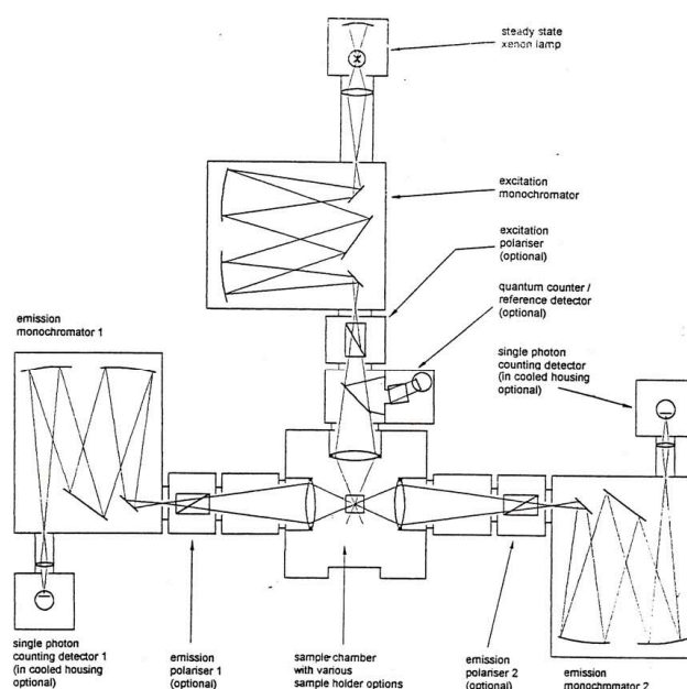
Figure 9: Optical layout of the spectrometer FS9000CDT
