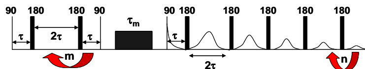
Fig. 1: The ARTDECO sequence was used to measure T_2 exchange. There are two CPMG [6] echo trains separated by an exchange time.
