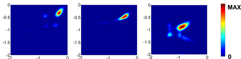
Fig. 2: Borosilicate glass beads saturated in water (left), in BHI-salt solution media (middle), and biofouled in BHI-salt solution media (right). All had a 1.0 s mixing time. The T_2 values for the main diagonal peaks shifted with the addition of media from 0.48 s to 0.30 s. After biofouling the bead pack in BHI-salt solution media T_2 values for the main diagonal peaks shifted further from 0.30 s to 0.12 s. Additionally, off diagonal peaks are visible which indicate exchange. The T_2 - T_2 maps are shown on a log-log scale.
