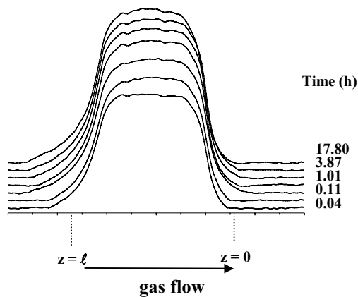
Fig. 5. 1D-NMR profiles of n-hexane adsorbed in HZSM5 zeolite in powder form.
