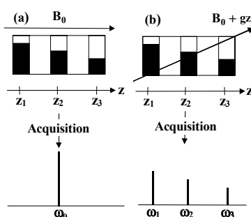
Fig. 1. Principle of 1D NMR Imaging
