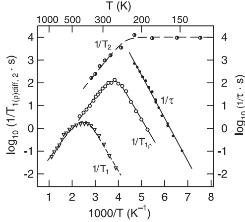
FIG. 2: Li jumps rates \tau^{-1} ( \bullet ) vs 1/T directly measured by SAE NMR in comparison with the T_{1\text{diff}}^{-1} ( \nabla 9.97 MHz) and T_{1\varrho\text{diff}}^{-1} ( \circ 5.2 kHz) data. The dashed and solid lines are fits according to the Richards expression (see text). Constant T_2^{-1} rates ( \bullet ) below 220 K mark the rigid lattice regime.
