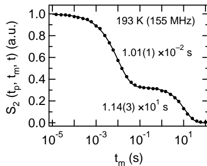
FIG. 1: Semilog plot of normalized {}^7\text{Li} SAE amplitudes of \text{Li}_{0.7}\text{TiS}_2 vs t_m ( t = t_p = 15 \mu\text{s} ) at 193 K. The first decay step directly yields the Li residence time \tau = 1.01(1) \times 10^{-2} s, whereas the second decay step simply reflects T_1 relaxation, T_1 \approx 1.1 \times 10^1 s. The solid line represents a fit according to the sum of a stretched ( \tau ) and a single exponential ( T_1 ).
