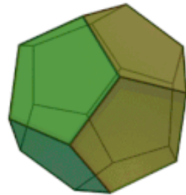
Dodekaeder – Kosmos
