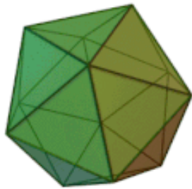
Ikosaeder – Wasser
