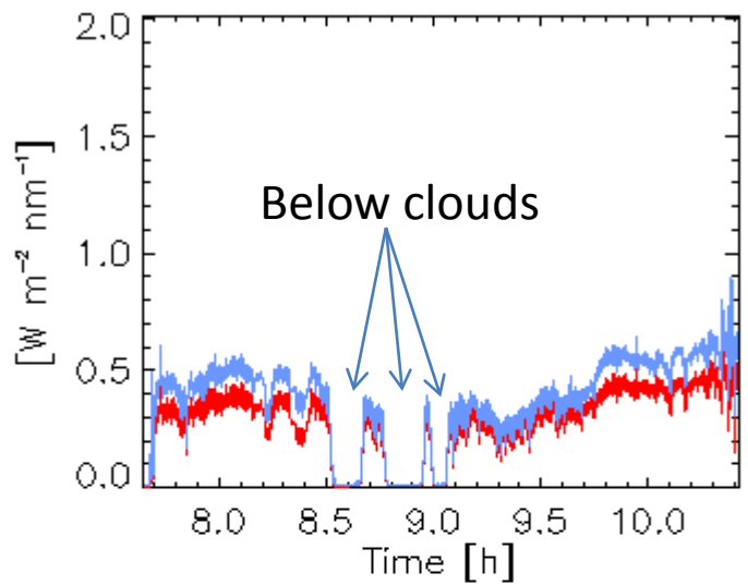
Upwelling Radiance
