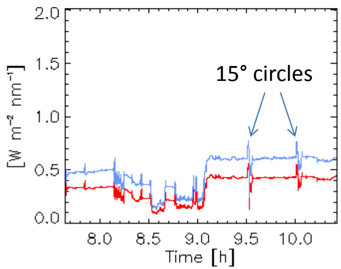
Downwelling Irradiance
