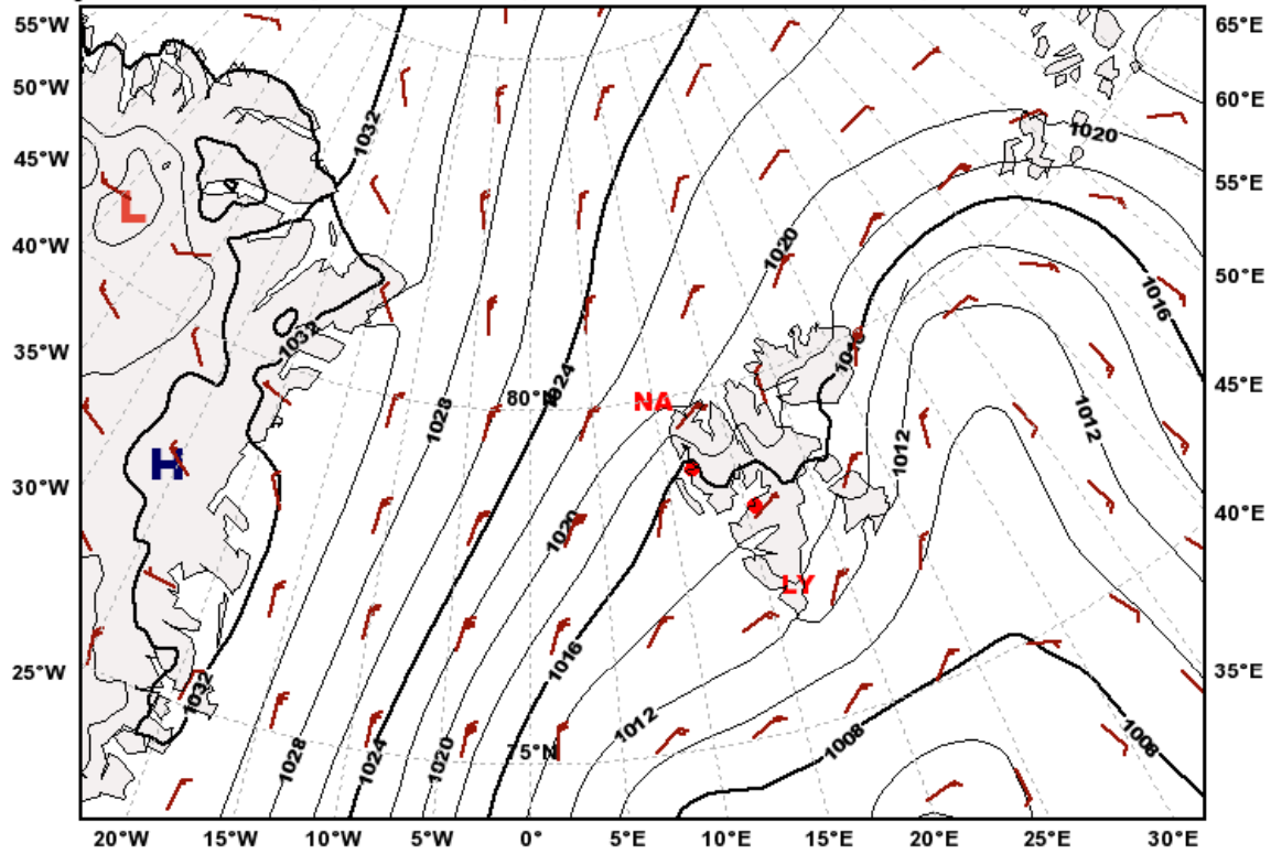
Mean Sea Level Pressure valid: Sun, 09 May 2010, 15 UTC (init: 20100509 00 UTC +015 h)
