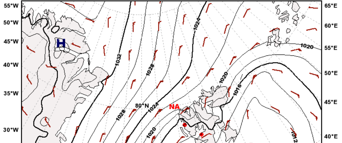
Mean Sea Level Pressure valid: Sun, 09 May 2010, 06 UTC (init: 20100509 00 UTC +006 h)
