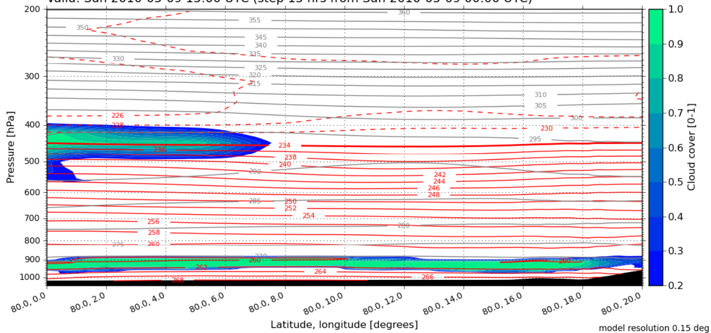
Cloud cover [0-1] with temperature [K] and potential temperature [K] Valid: Sun 2010-05-09 15:00 UTC (step 15 hrs from Sun 2010-05-09 00:00 UTC)
