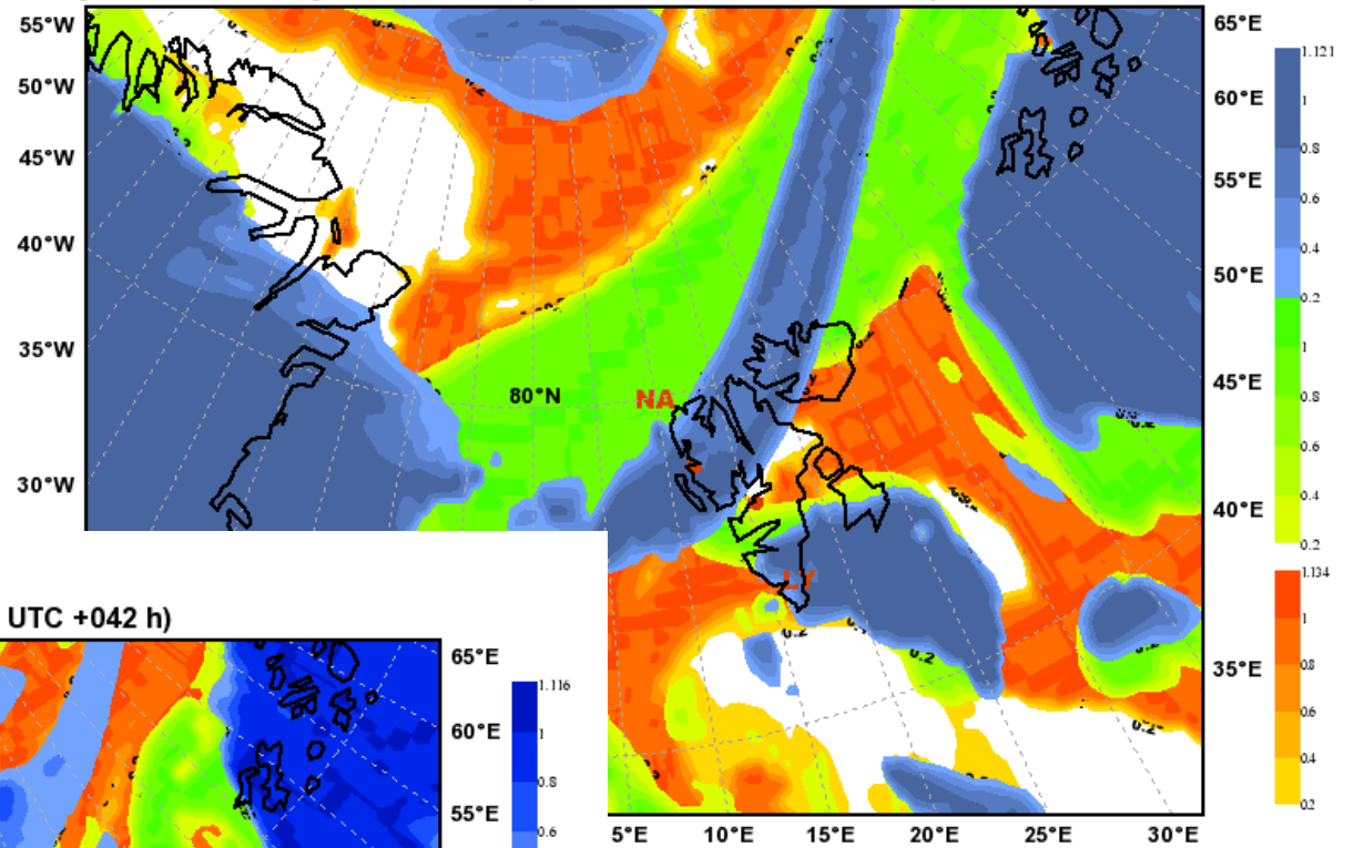
Total Cloud Cover Valid: Thu, 13 May 2010, 06 UTC (init: 20100512 00 UTC +030 h)
