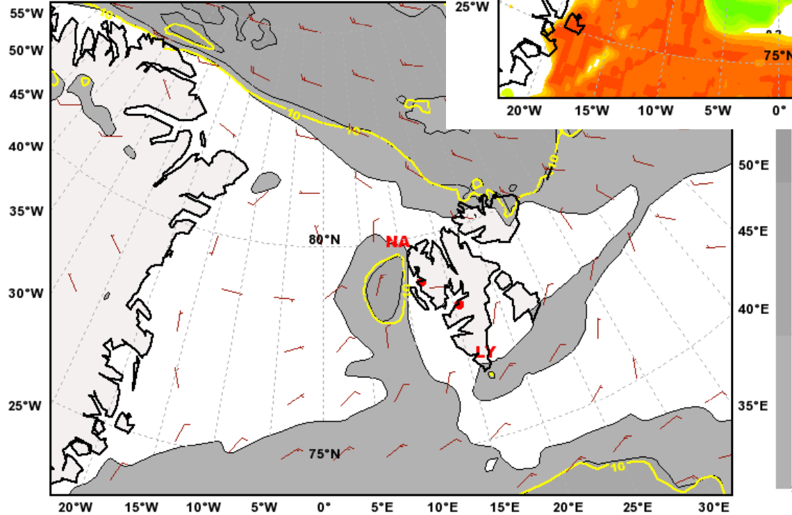
10 m Wind and 10 m Wind gusts [m s -1 ] Valid: Fri, 14 May 2010, 12 UTC (init: 20100512 00 UTC +060 h)
