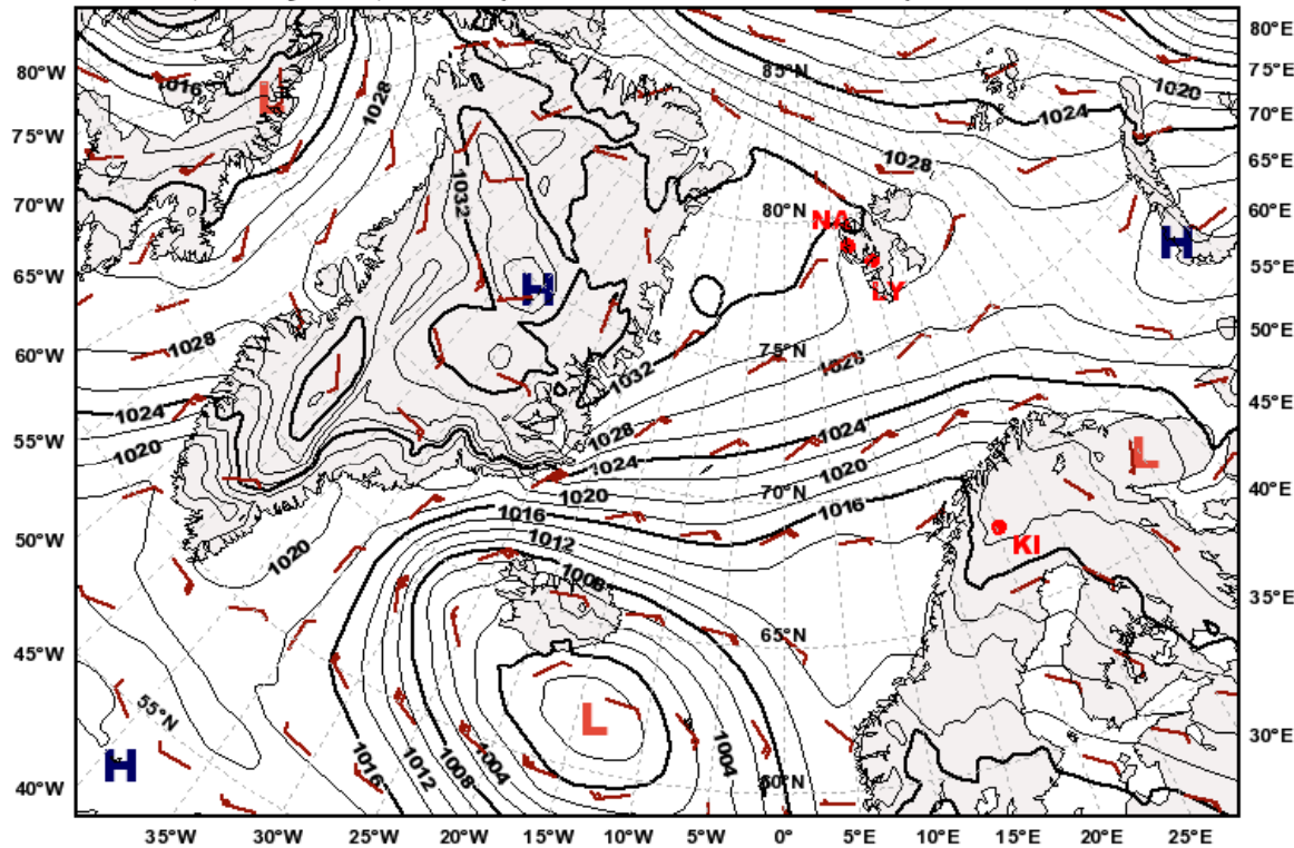
Mean Sea Level Pressure valid: Fri, 14 May 2010, 12 UTC (init: 20100512 00 UTC +060 h)
