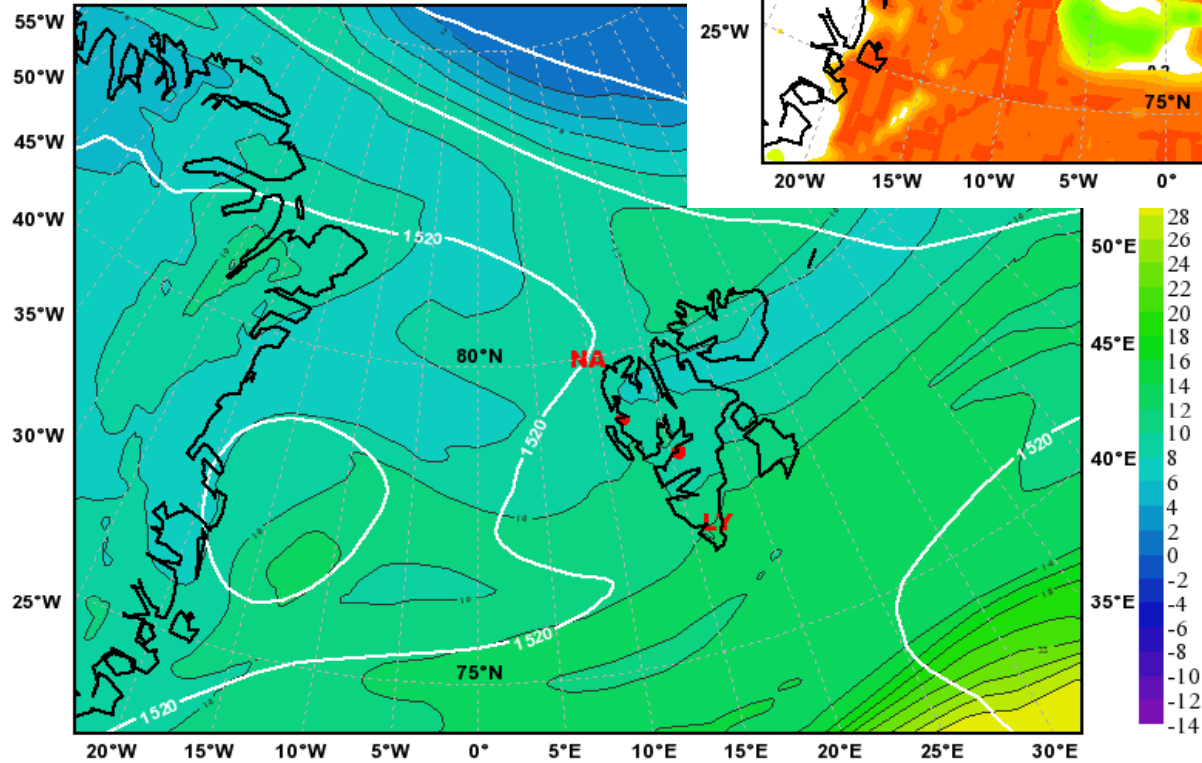
Equivalent Potential Temperature [°C] & Geopot. H Valid: Fri, 14 May 2010, 12 UTC (init: 20100512 00 UTC +060 h)
