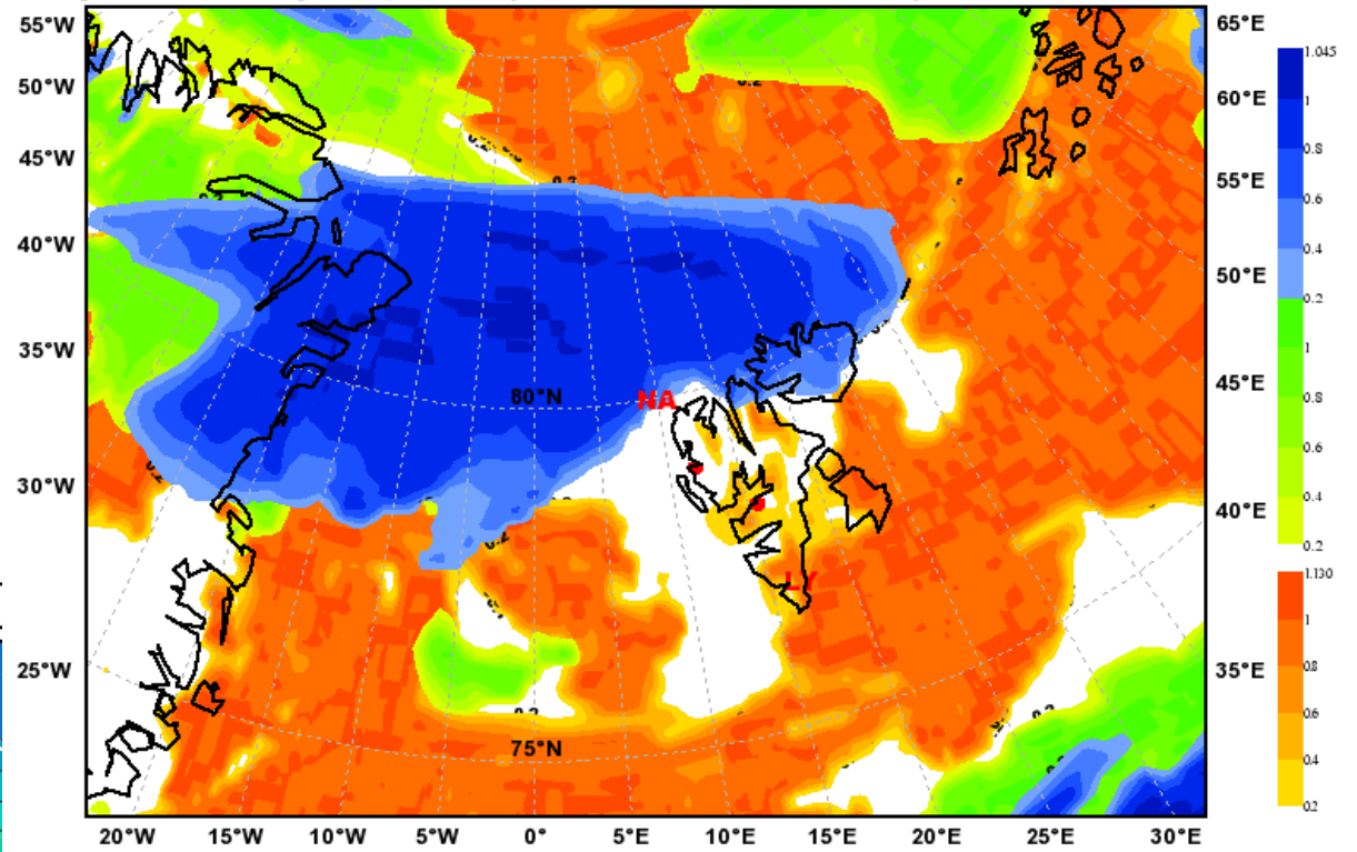
Total Cloud Cover Valid: Fri, 14 May 2010, 12 UTC (init: 20100512 00 UTC +060 h)
