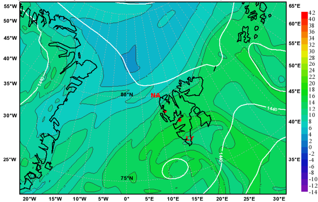
Equivalent Potential Temperature [°C] & Geopot. Height [m] at 850hPa Valid: Thu, 13 May 2010, 12 UTC (init: 20100512 00 UTC +036 h)
