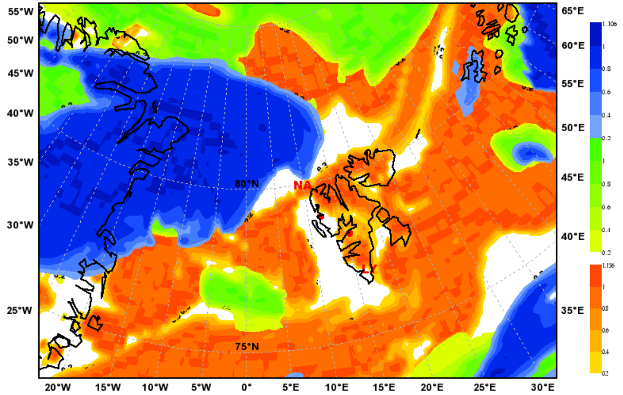
Total Cloud Cover Valid: Fri, 14 May 2010, 06 UTC (init: 20100512 00 UTC +054 h)
