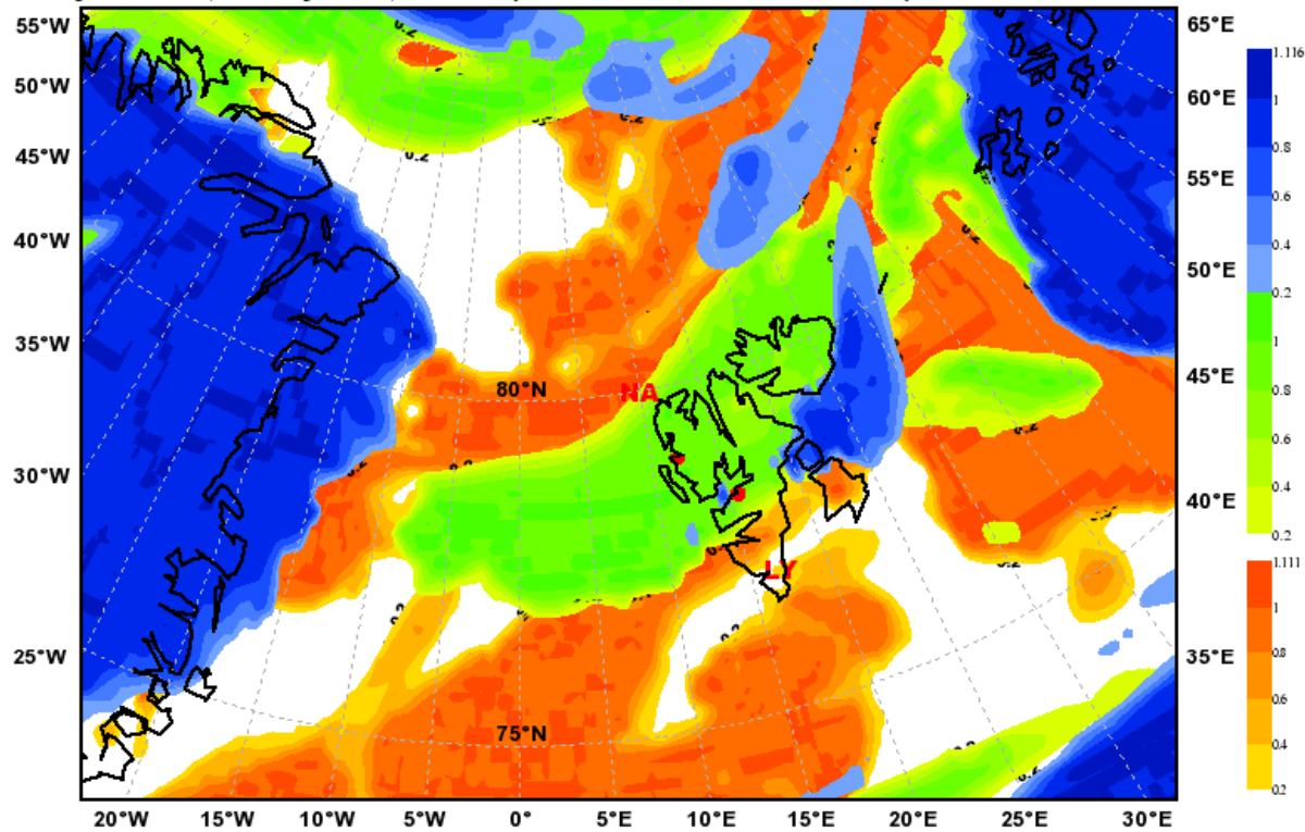
Total Cloud Cover Valid: Thu, 13 May 2010, 18 UTC (init: 20100512 00 UTC +042 h)
