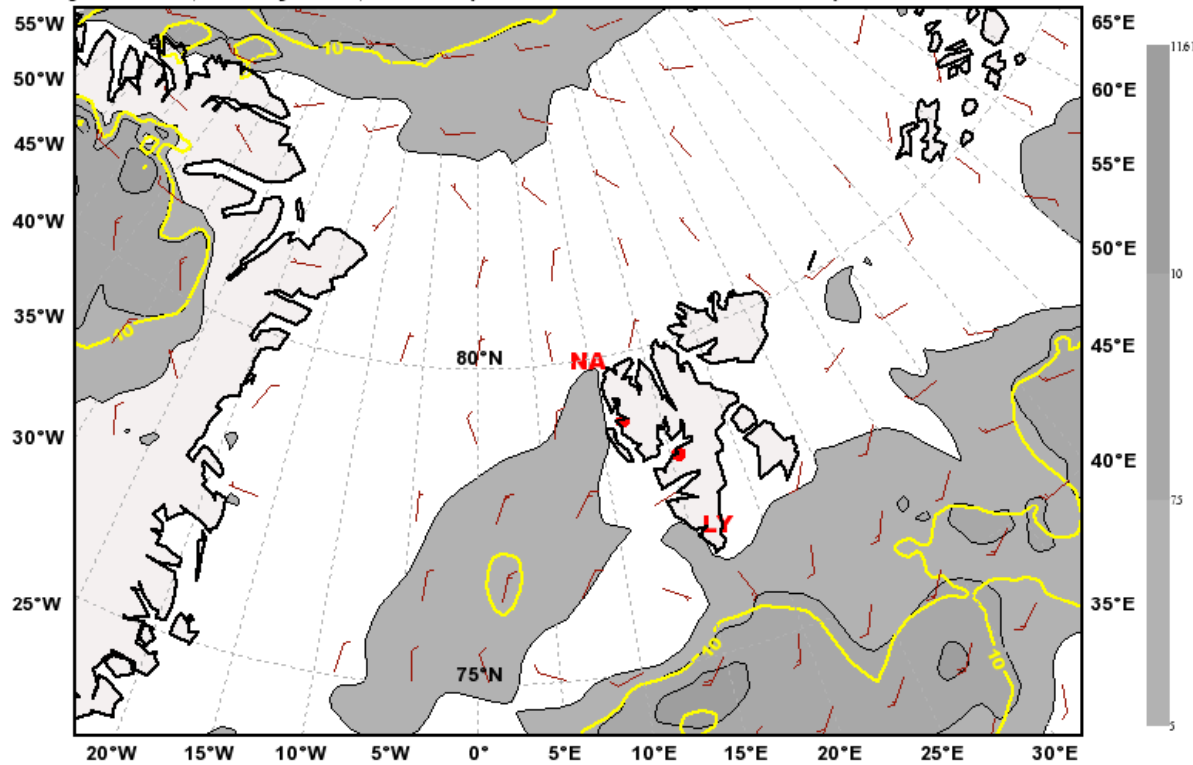
10 m Wind and 10 m Wind gusts [m s -1 ] Valid: Thu, 13 May 2010, 12 UTC (init: 20100512 00 UTC +036 h)
