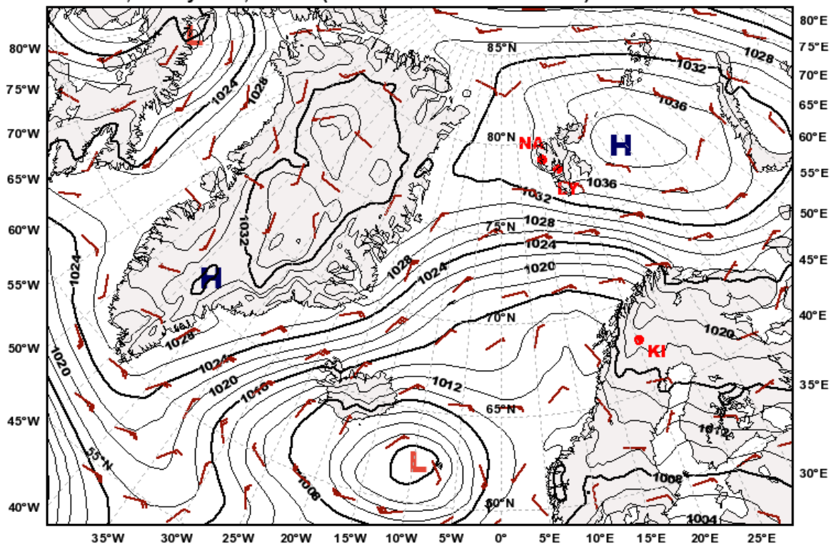
Mean Sea Level Pressure valid: Sat, 15 May 2010, 12 UTC (init: 20100513 00 UTC +060 h)
