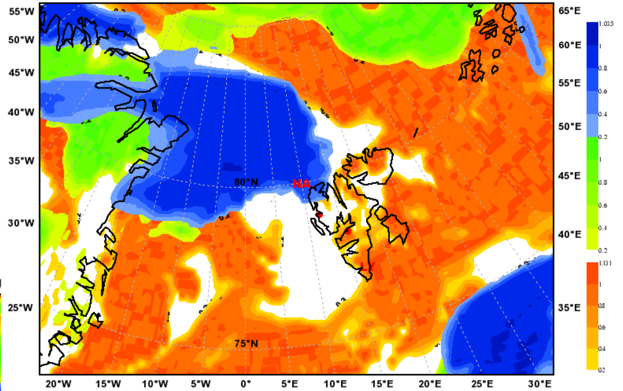
Total Cloud Cover Valid: Fri, 14 May 2010, 12 UTC (init: 20100513 00 UTC +036 h)
