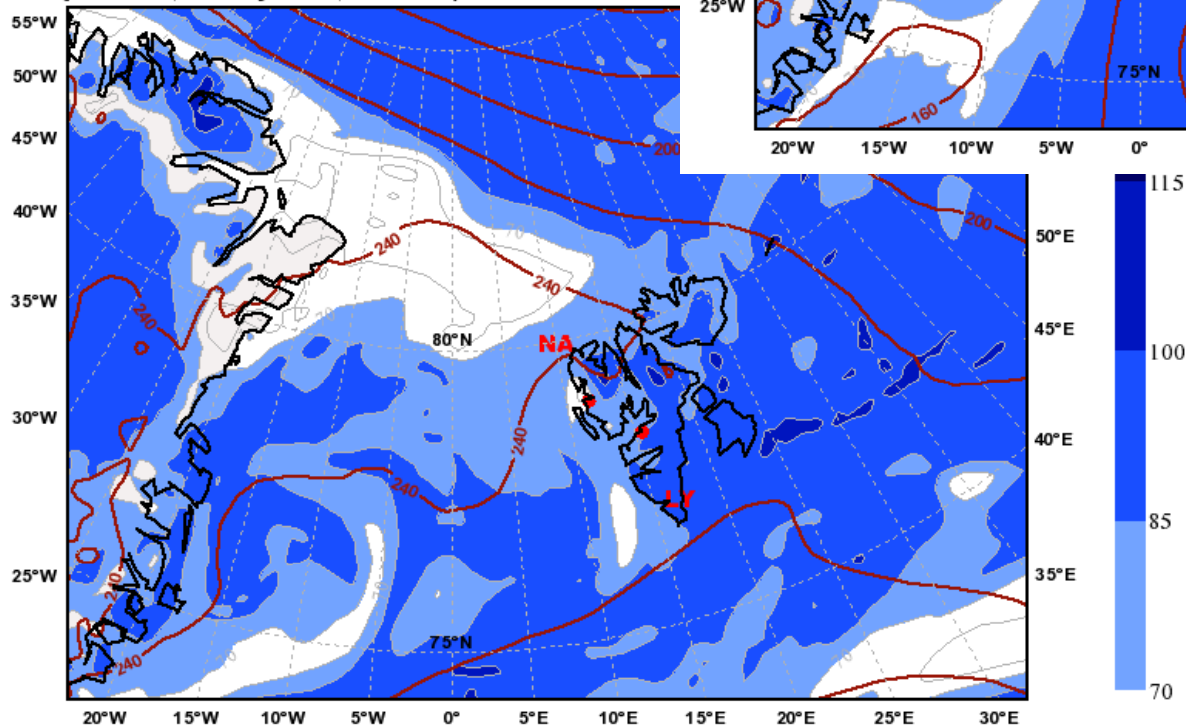
Relative Humidity [%] and Geopotential Height [m] valid: Fri, 14 May 2010, 09 UTC (init: 20100513 00 UTC +012 h)
