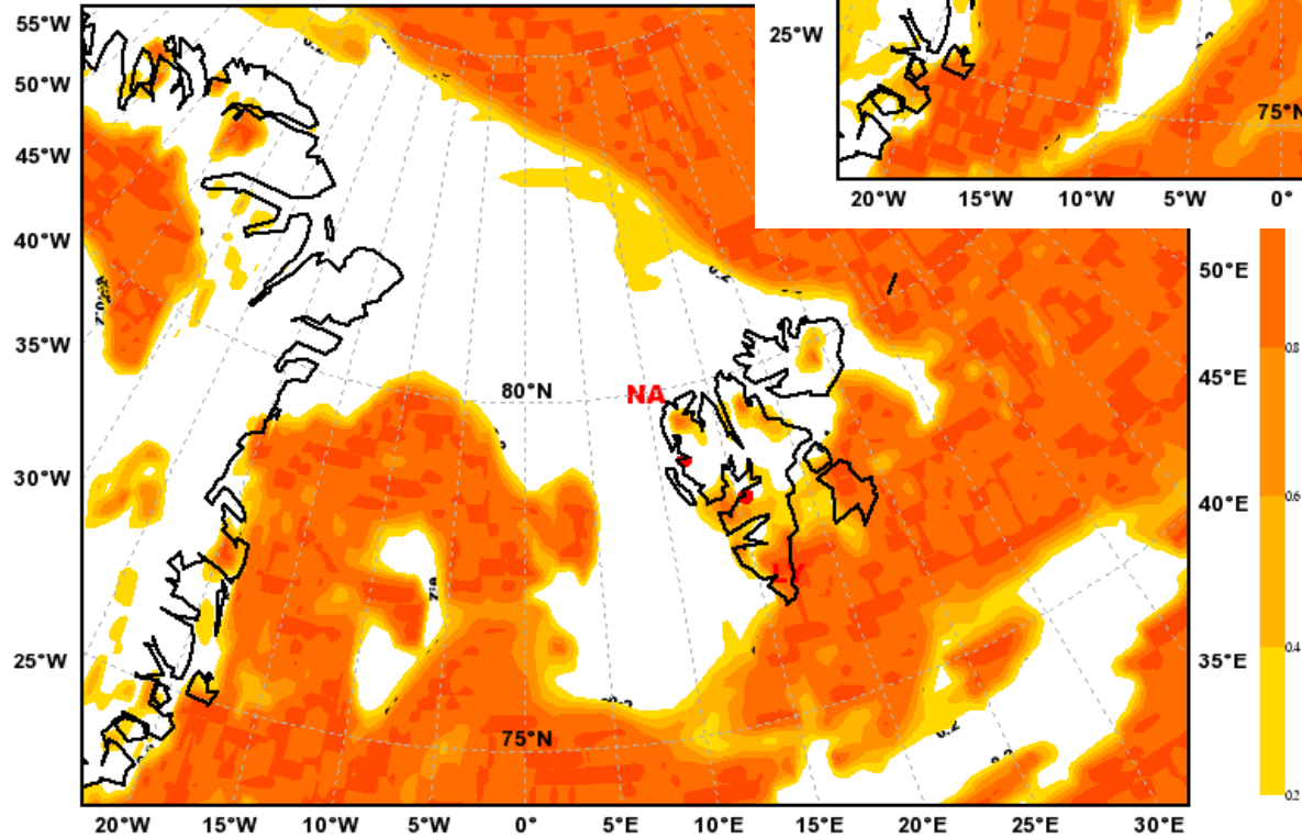
Low Cloud Cover Valid: Fri, 14 May 2010, 15 UTC (init: 20100513 00 UTC +033 h)
