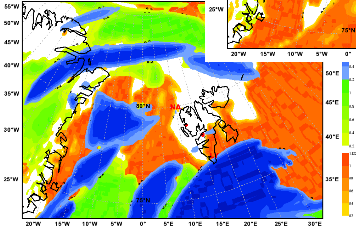
Total Cloud Cover Valid: Sat, 15 May 2010, 12 UTC (init: 20100513 00 UTC +036 h)
