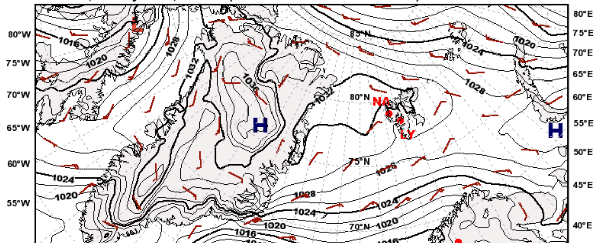
Mean Sea Level Pressure valid: Fri, 14 May 2010, 12 UTC (init: 20100513 00 UTC +036 h)
