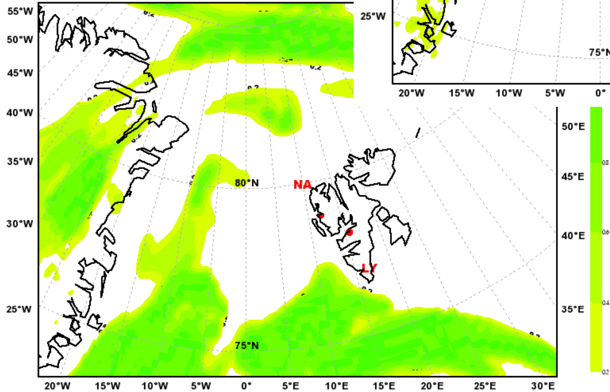
Medium Cloud Cover Valid: Sat, 15 May 2010, 15 UTC (init: 20100513 00 UTC +033 h)
