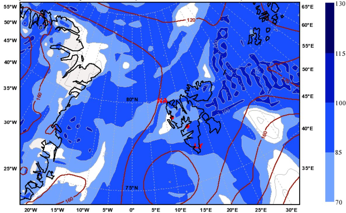
Relative Humidity [%] and Geopotential Height [m] at 1000hPa valid: Thu, 13 May 2010, 12 UTC (init: 20100513 00 UTC +012 h)
