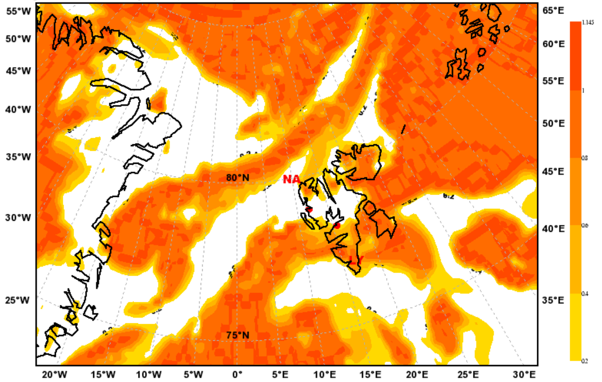
Low Cloud Cover Valid: Thu, 13 May 2010, 12 UTC (init: 20100513 00 UTC +012 h)
