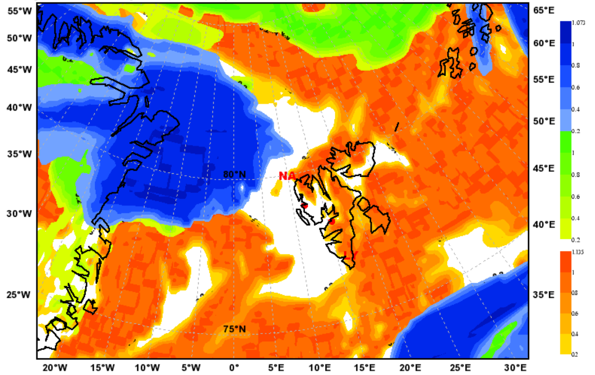
Total Cloud Cover Valid: Fri, 14 May 2010, 09 UTC (init: 20100513 00 UTC +033 h)
