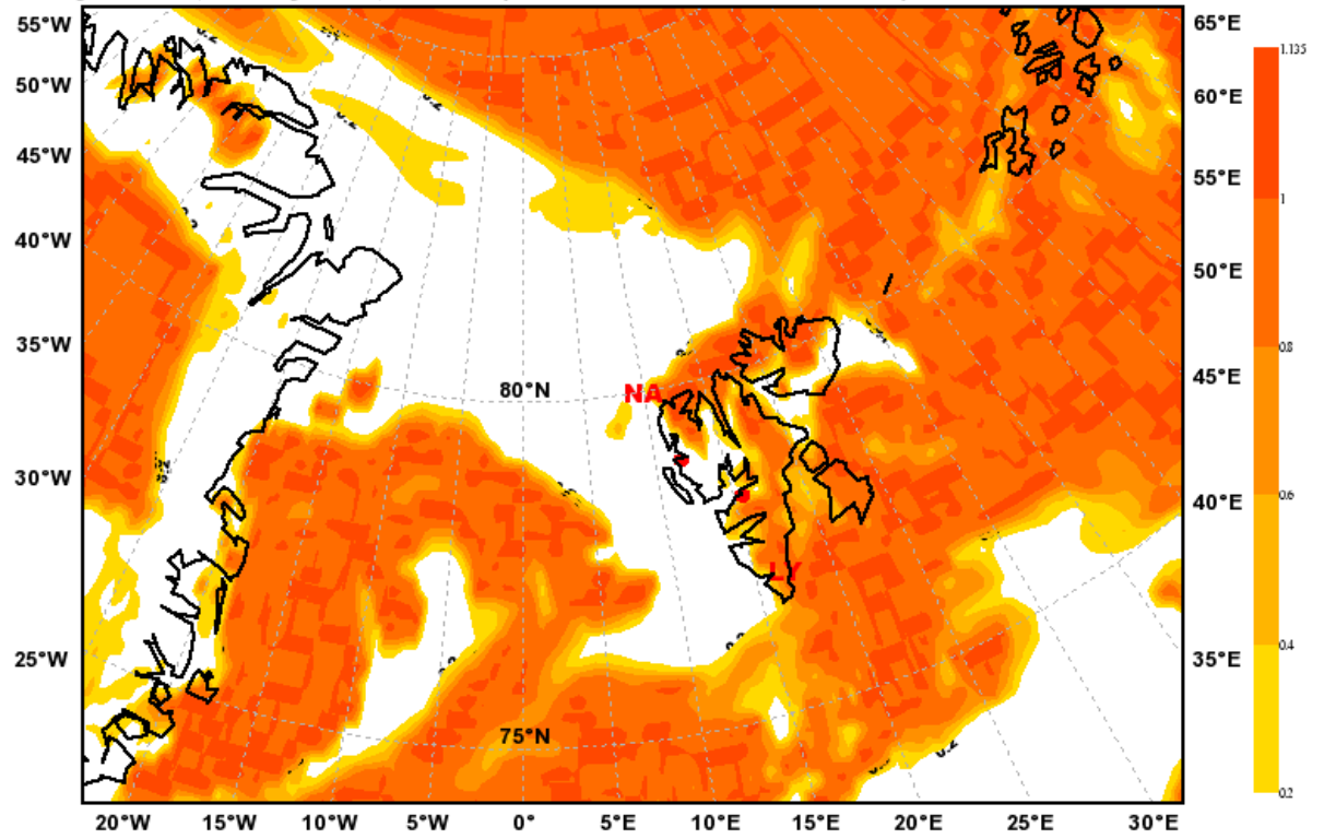
Low Cloud Cover Valid: Fri, 14 May 2010, 09 UTC (init: 20100513 00 UTC +033 h)
