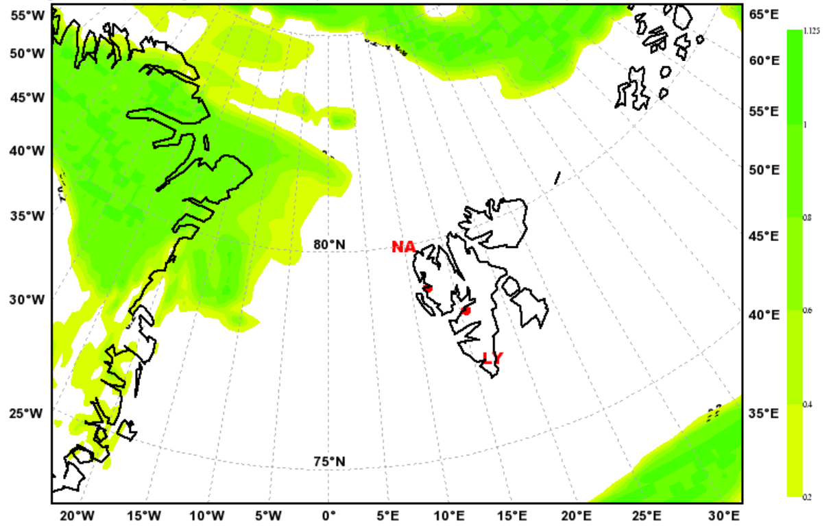
Medium Cloud Cover Valid: Fri, 14 May 2010, 09 UTC (init: 20100513 00 UTC +033 h)
