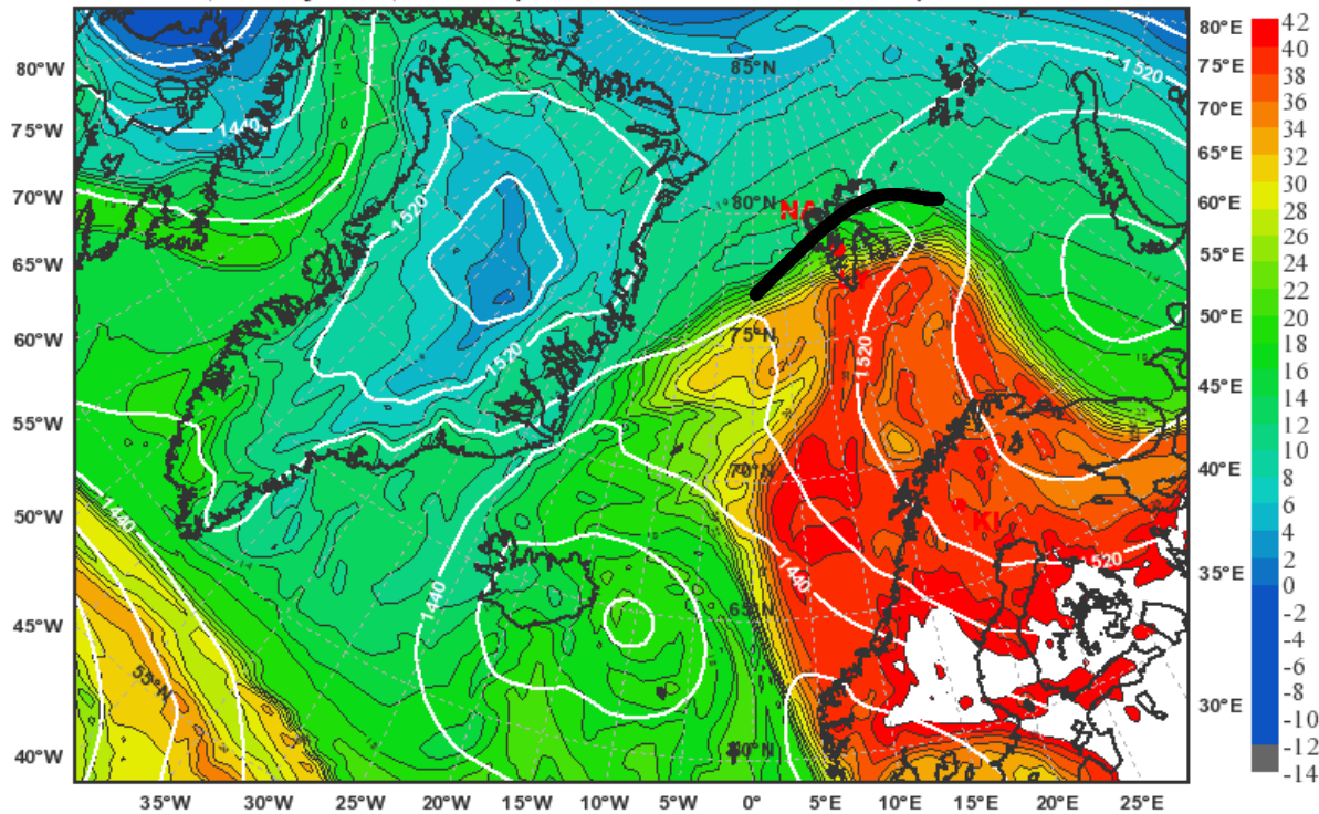
Equivalent Potential Temperature [°C] & Geopot. Height [m] at 850hPa valid: Sun, 16 May 2010, 12 UTC (init: 20100514 00 UTC +060 h)
