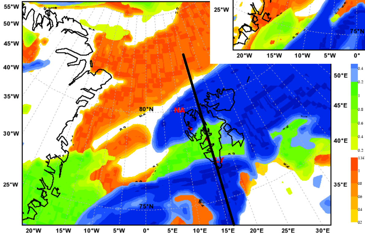
Total Cloud Cover Valid: Sun, 16 May 2010, 12 UTC (init: 20100514 00)
