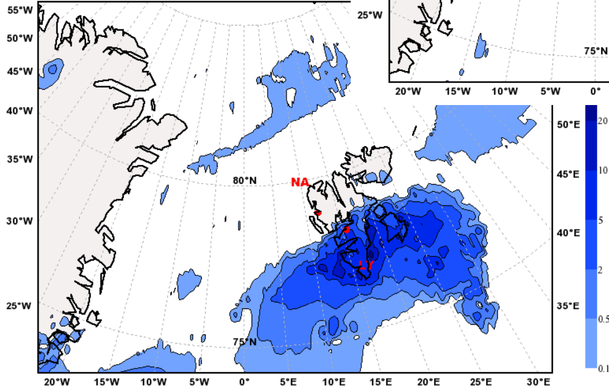
Total Precipitation [mm] Valid: Sun, 16 May 2010, 03-09 UTC (init: 20100514)
