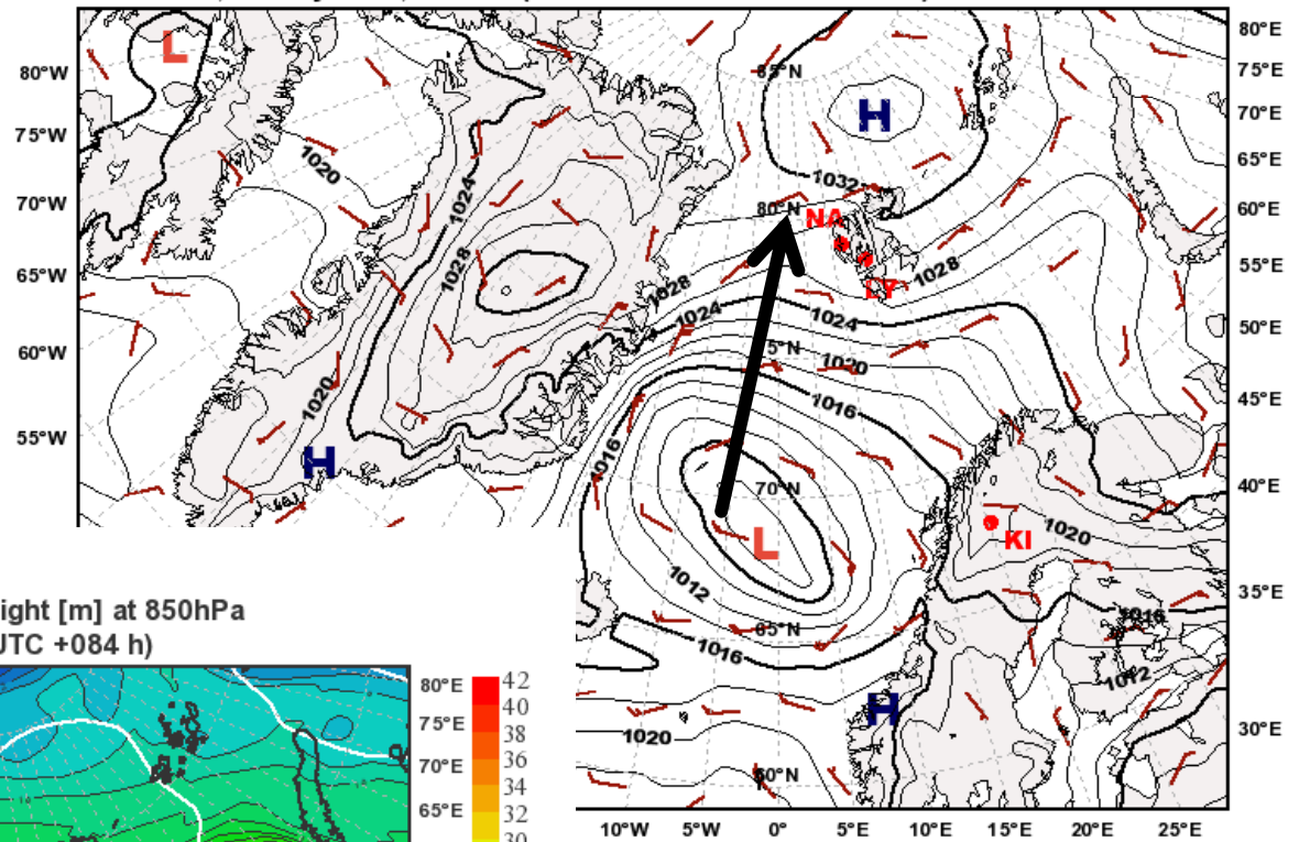
Mean Sea Level Pressure valid: Mon, 17 May 2010, 12 UTC (init: 20100514 00 UTC +084 h)
