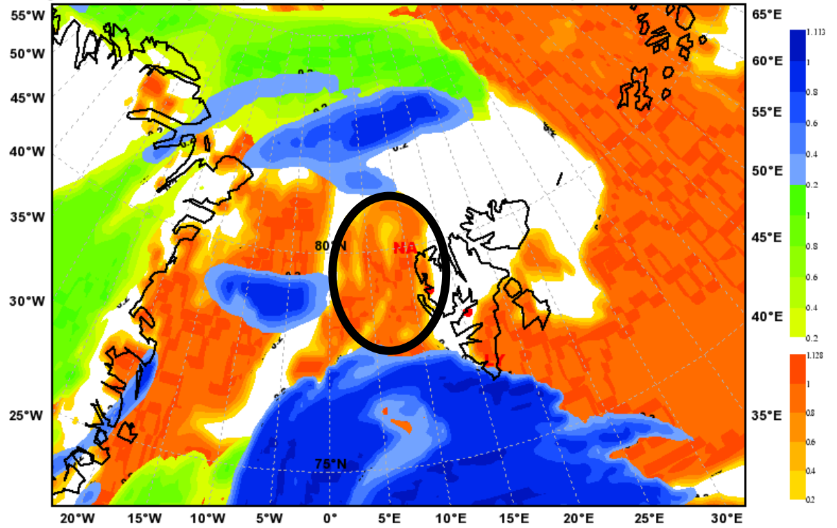
Total Cloud Cover Valid: Sat, 15 May 2010, 09 UTC (init: 20100514 00 UTC +033 h)
