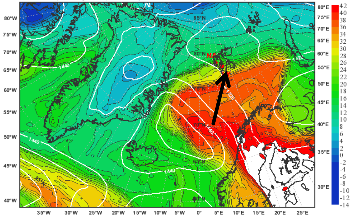
Equivalent Potential Temperature [°C] & Geopot. Height [m] at 850hPa valid: Mon, 17 May 2010, 12 UTC (init: 20100514 00 UTC +084 h)
