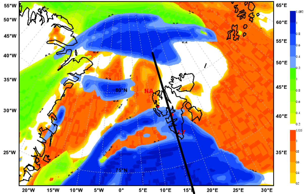
Total Cloud Cover Valid: Sat, 15 May 2010, 12 UTC (init: 20100514 00 UTC +036 h)
