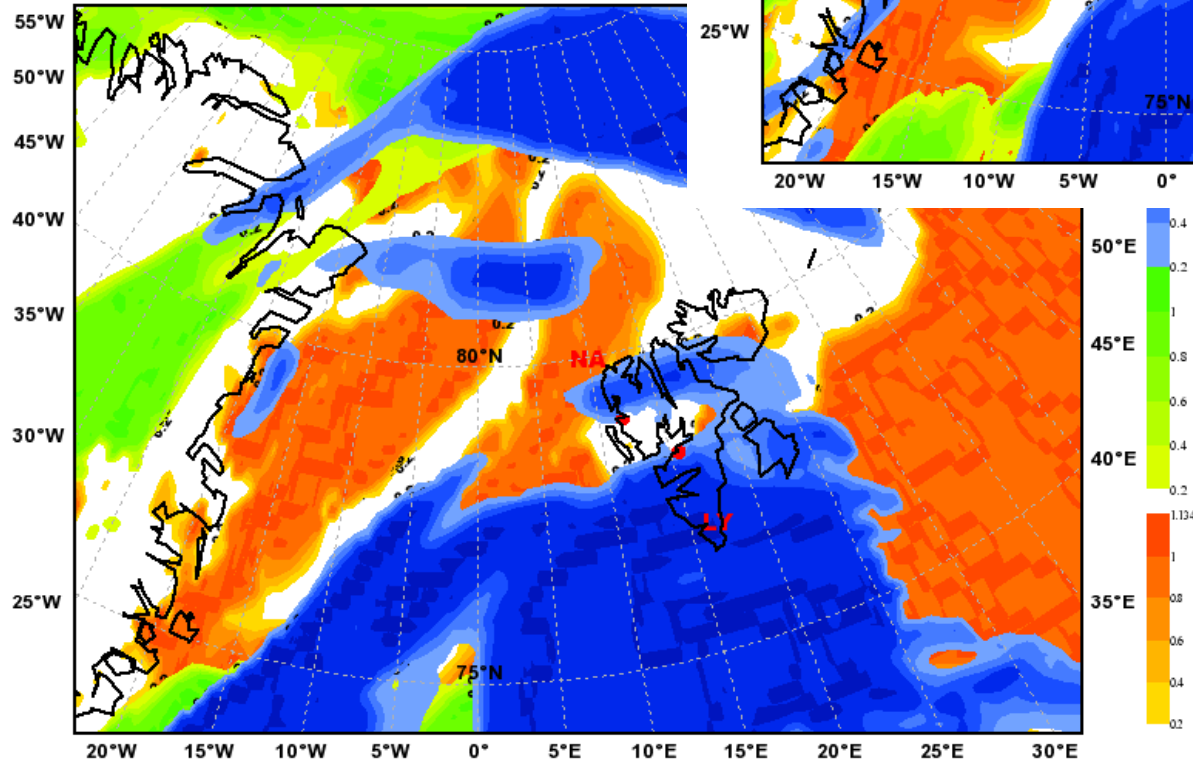
Total Cloud Cover Valid: Sat, 15 May 2010, 15 UTC (init: 20100514 00 UTC +033 h)
