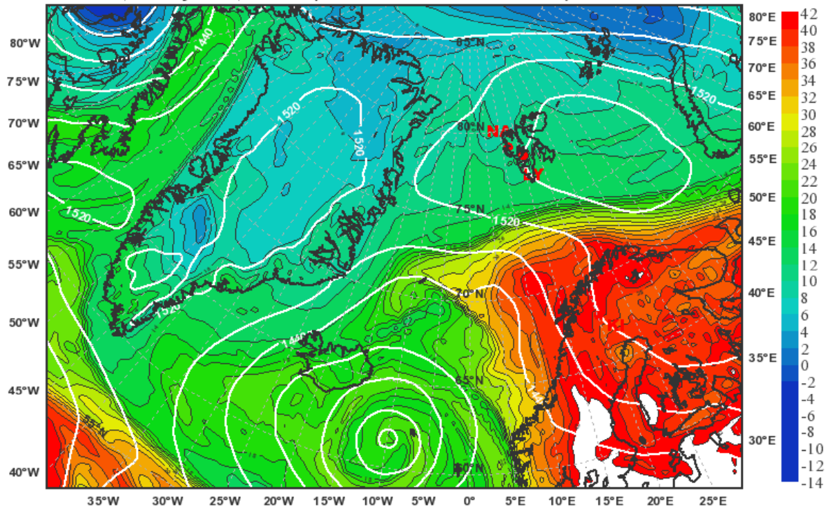
Equivalent Potential Temperature [°C] & Geopot. Height [m] at 850hPa valid: Sat, 15 May 2010, 12 UTC (init: 20100514 00 UTC +036 h)
