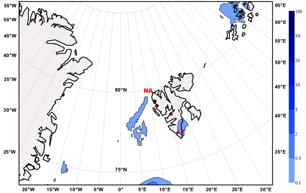
Total Precipitation [mm] Valid: Sat, 15 May 2010, 12-15 UTC (init: 20100514 00 UTC +039 h)
