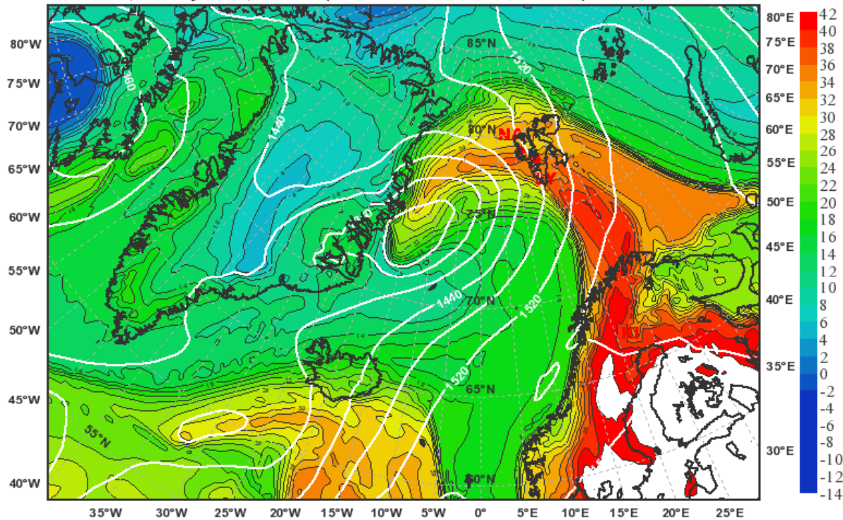
Equivalent Potential Temperature [°C] & Geopot. Height [m] at 850hPa valid: Tue, 18 May 2010, 12 UTC (init: 20100514 00 UTC +108 h)
