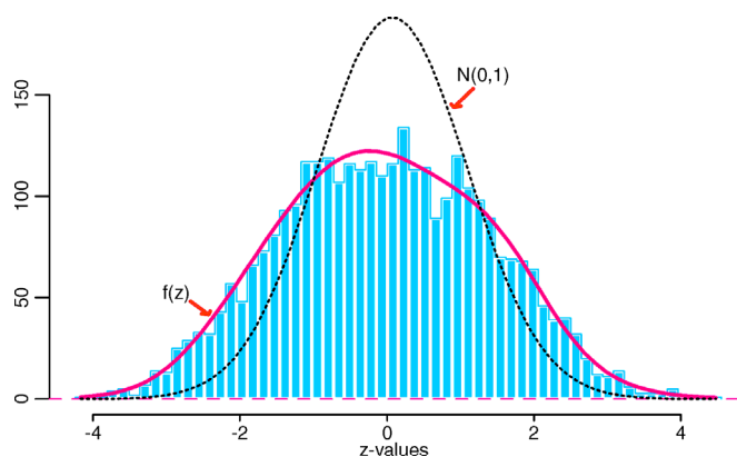
Figure 6. Histogram of N = 3,226 z -Values From the Breast Cancer Study. The theoretical N(0, 1) null is much narrower than the central peak, which has (\delta_0, \sigma_0) = (-.02, 1.58) . In this case the central peak seems to include the entire histogram.
