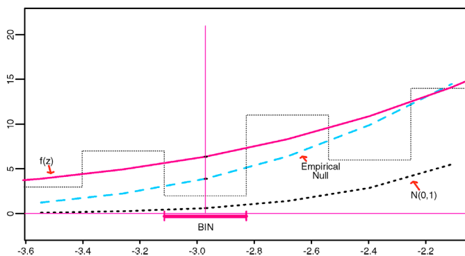
Figure 2. Close-Up View of the Bin Containing z = -3 in Figure 1. Expected numbers in the bin are 6.37 for f(z) , .62 for f_0 = N(0, 1) , and 3.90 for f_0 = N(-.35, 1.20^2) , the empirical null. Corresponding estimates of \text{fdr}(-3) are .097 for N(0, 1) versus .612 for N(-.35, 1.20^2) . Should we report the cases in this bin as Interesting?
