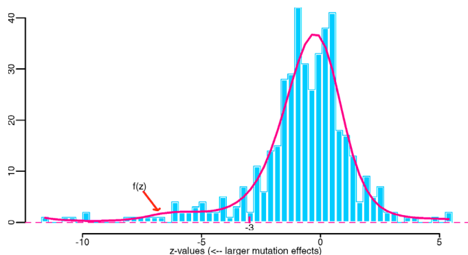
Figure 1. Histogram of 444 z-Values From the Drug Mutation Analysis. The smooth curve f(z) is a natural spline fit to histogram counts. The central peak near z = 0 is approximately N(-.35, 1.20^2) , the “empirical null hypothesis.” Simultaneous hypothesis tests for the 444 cases depend critically on the choice between the empirical or theoretical N(0, 1) null.
